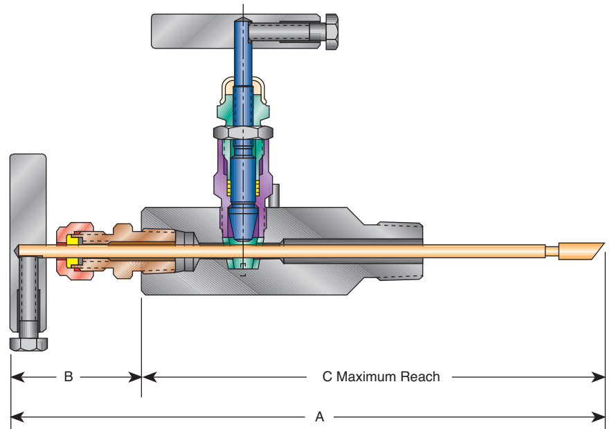
Rod-Out Device with M5 Gauge Valve
